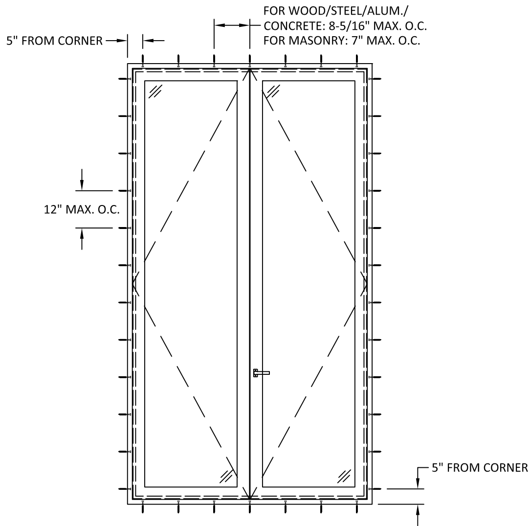
ANCHOR LAYOUT FRENCH DOOR
