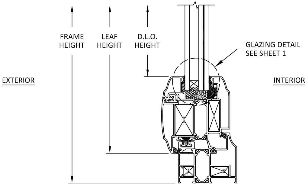
B 4 VERTICAL SECTION SILL
