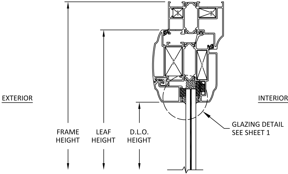
A 4 VERTICAL SECTION HEAD
