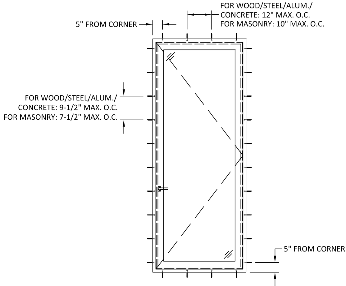
ANCHOR LAYOUT SINGLE DOOR
